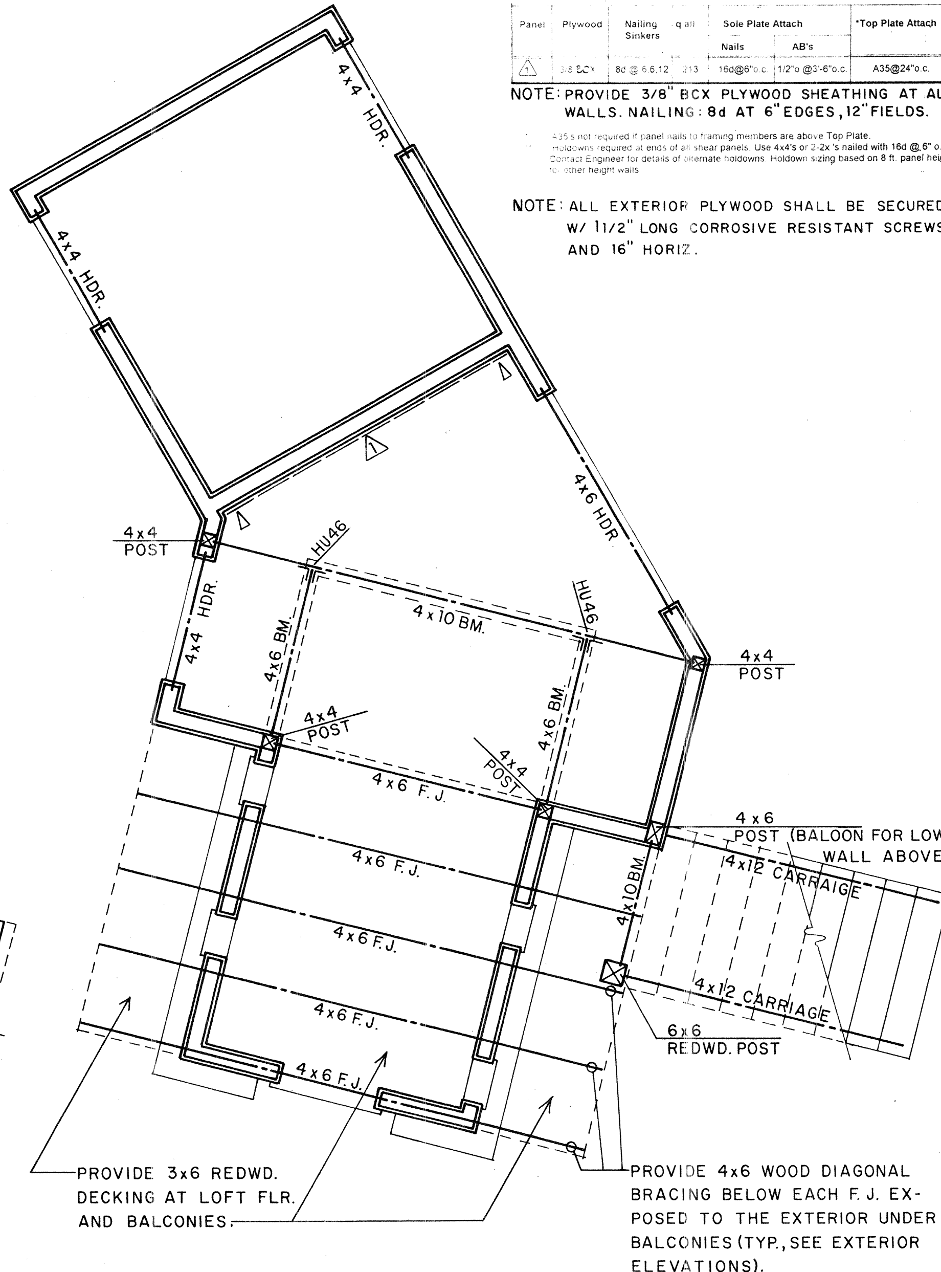
FRAMING PLAN 1/2" = 1'-0" north
