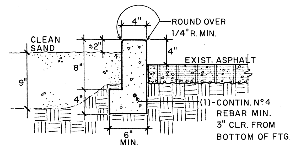
1 UNDULATING CURB DETAIL 1/2" = 1'-0"
