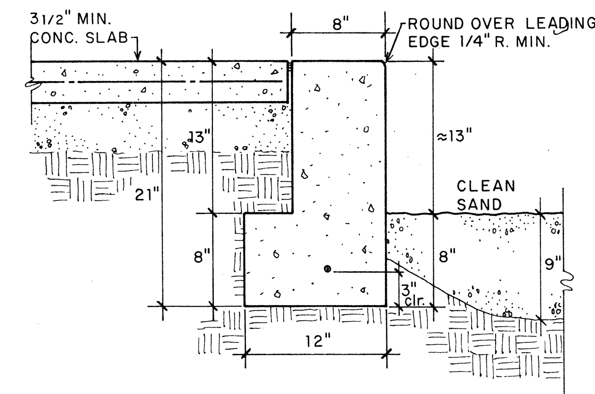
4 WALL DETAIL 1/2" = 1'-0"
