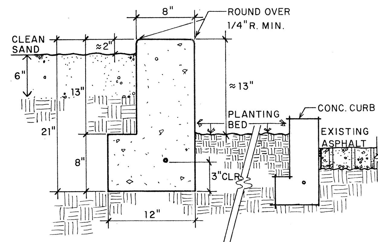
2 WALL DETAIL 1/2" = 1'-0"
