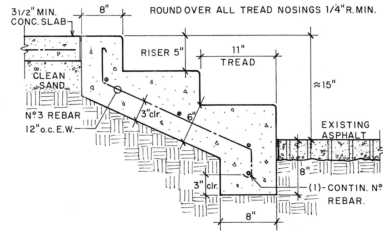
3 CONCRETE STAIR DETAIL 1/2" = 1'-0"
